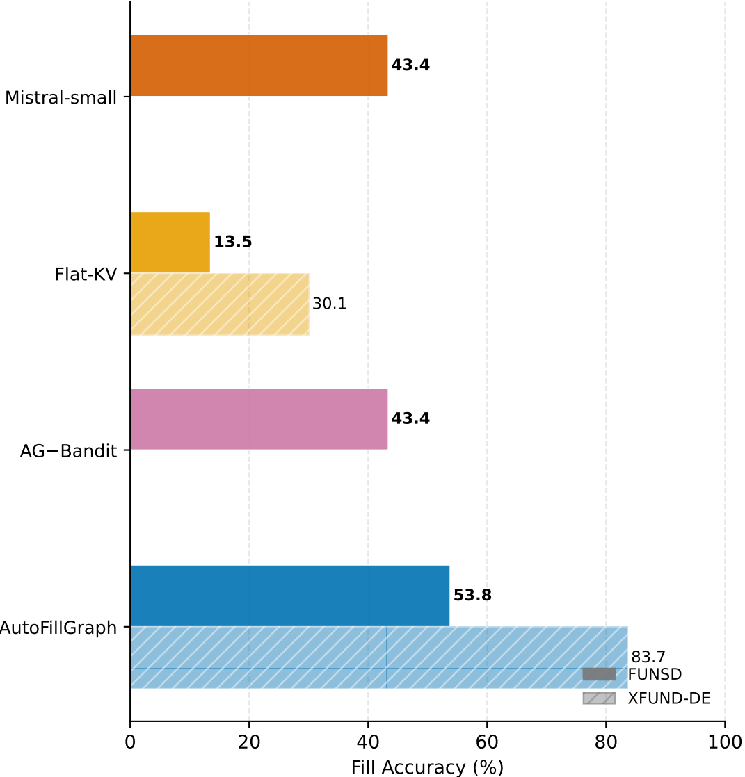
Fill Accuracy — All Systems
